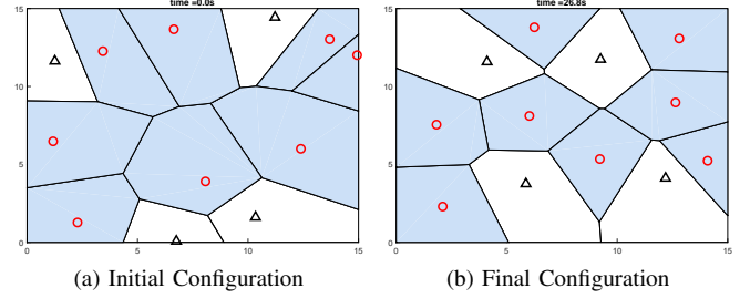
Figure 2: Symmetry trap when pursuers (triangles) attempt to minimize the area of all evaders (circles). The pursuers get trapped in the final configuration.
