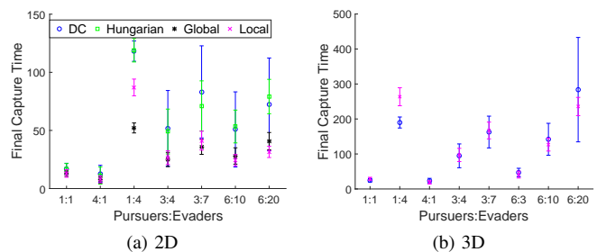
Figure 5: Mean final capture time for the pursuer policies in Table I over randomized trials. The local area-minimization policy from Algorithm 2 is shown in pink x's.
