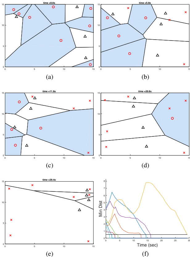
Figure 3: (a)-(e) Simulation of 4 pursuers (triangles) and 8 evaders (circles), with captured evaders as x's and safe-reachable area shaded. (f) Minimum distance over time of evaders to any pursuer, with capture radius marked in black.
