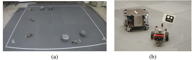
Figure 1: Experiments were conducted using Oujabot pursuers and GoPiGo evaders. The evaders are always captured, even when they are controlled by a human operator.
