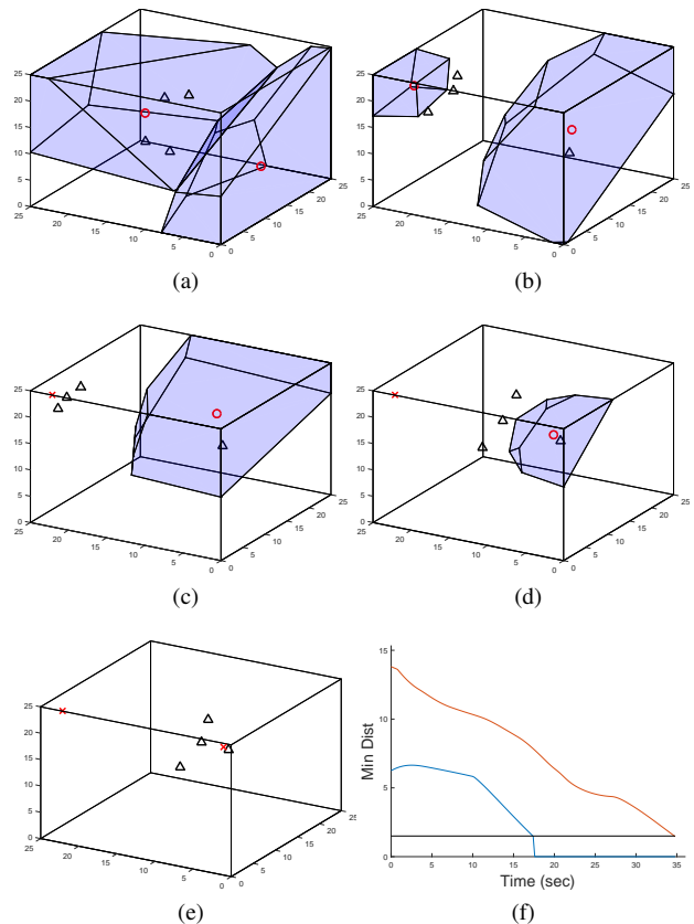
Figure 4: (a)-(e) Simulation of 4 pursuers (triangles) and 2 evaders (circles), with captured evaders as x's and the safe-reachable area shaded. (f) Minimum distance over time of evaders to any pursuer, with capture radius marked in black.
