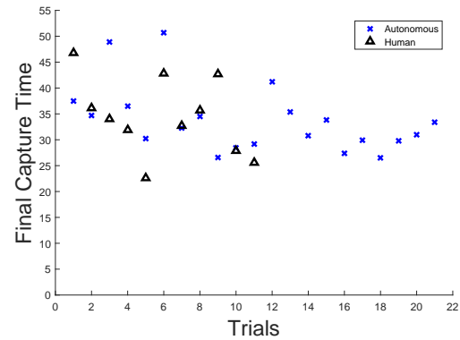
Figure 11: Final capture time of evaders over different trials. All-autonomous trials are marked with x's and human-evader trials with triangles.
